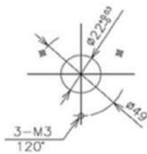
Servo Mount
