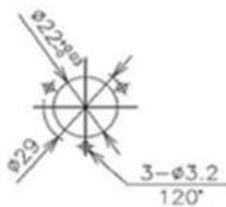
Screw Mount
